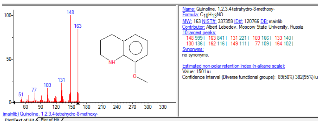
სურ.8 1,2,3,4-Tetrahydro-8-methoxyquinoline
