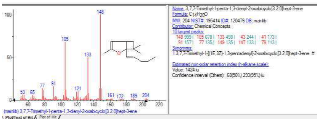
სურ.7 3,7,7-Trimethyl-1-(penta-1,3-dienyl)-2-oxabicyclo[3.2.0]hept-3-ene
